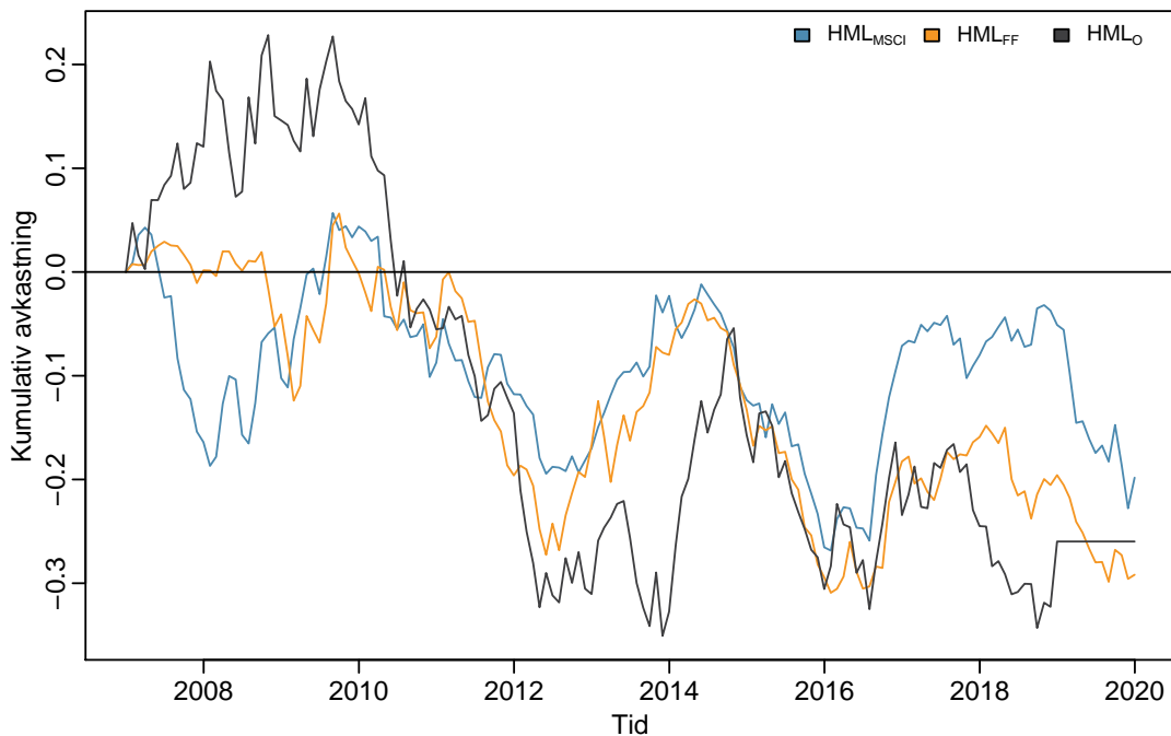
Figur C.5: HML-faktorer
