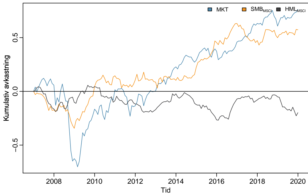
Figur C.1: Norden-faktorer
